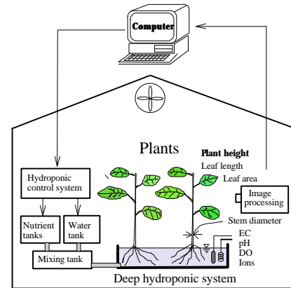
Fig 3 Hydroponic system control based on the SPA.
