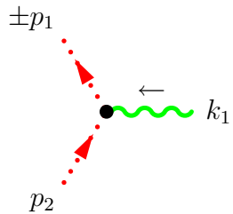
(f) One-Gluon - Ghost Vertex. (A.52) on page 130.
