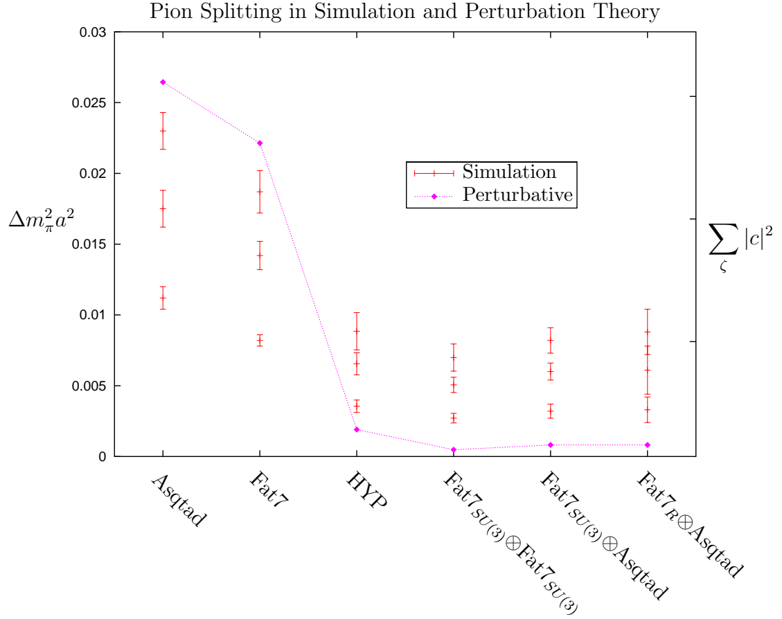
Figure 3.4: Quenched, m_0 = 0.03 , \beta = 5.93 splittings of m_\pi^2 for the 1-, 2- and 3-link tasteful mesons above the Goldstone pion for various quark actions with Wilson glue. On a different scale a measure of the one-loop perturbative taste-changing effects, \sum_\zeta |c|^2 is also shown which qualitatively explains the non-perturbative pion splittings; verifying that taste-changing can be understood as an \mathcal{O}(a^2\alpha_s^2) perturbative process. The proposed action \text{Fat7}_R \otimes \text{Asqtad} , shown on the right, has scaling violations due to taste-changing interactions about twice as small as the previous action, \text{Asqtad} , shown on the left.
