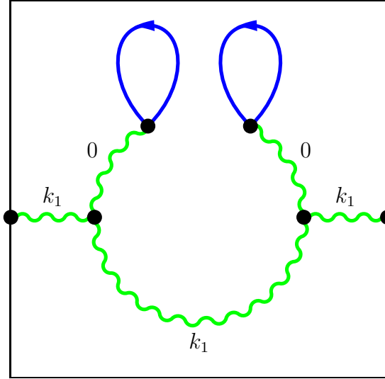
Figure 2.2: A disconnected diagram that can be very easily caught because it fails both criterion. It has four propagators with momenta of 0, one internal propagator with an “external” momenta from the expectation operator (not 1PI) and only one independent momenta, k_1 , not three.
