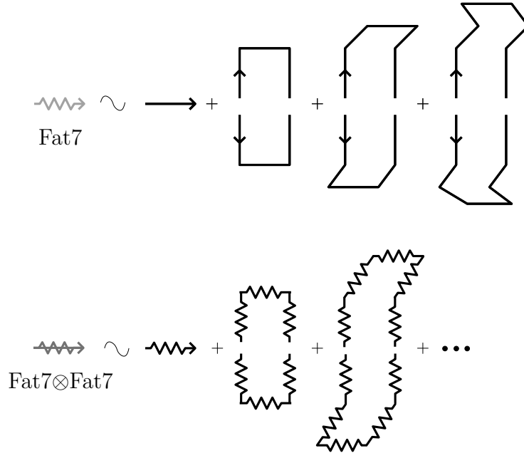
Figure 3.3: A schematic of Fat7 smearing (2.26b), and the principle behind smeared-smearings: the original smeared links are used in the second smearing. The \sim is because appropriate coefficients and sums over all directions of the path elements are not shown.
