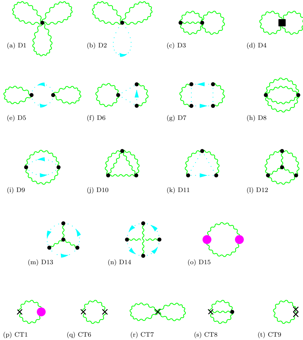
Figure 5.8: The three-loop pure glue Feynman diagrams for the expectation of a Wilson loop, evaluated from derivatives of vacuum bubbles using the susceptibility method (5.45). The magenta vertex is the amputated one-loop gluon propagator of figure 5.7. The diagram numbering is consistent with [72]. The lattice counter-terms are shown separately. The square vertex g^4 A^4 comes from the measure, and the cross, [double-cross] from \mathcal{O}(\alpha_{\text{lat}}^{[2]}) terms in the action.
