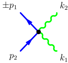
(c) Two Gluon - Quark Vertex. (A.47) on page 128.
