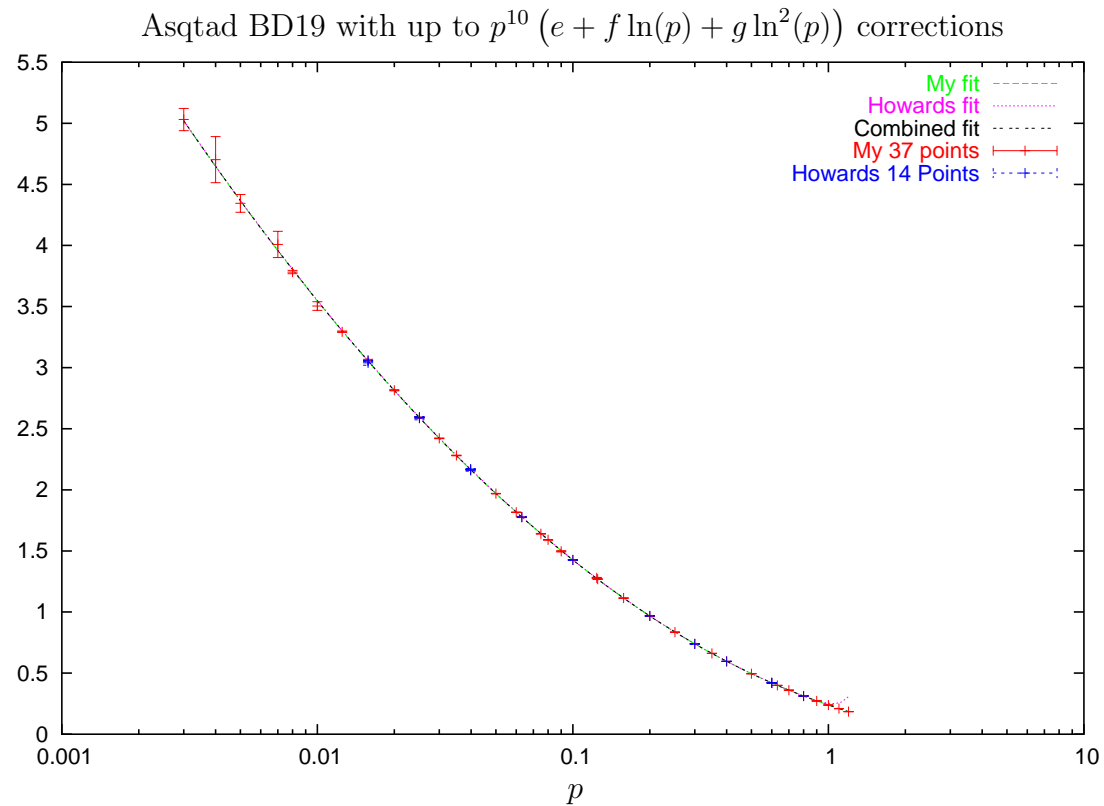
Figure 5.4: A sample fit for gluon diagram 19 in figure 5.3, one of the noisest, against the external momentum p in a semi-log plot. The curvature is the double logarithm with coefficient 3\frac{3}{8} , and the constant, logarithm and artifacts are fit for. The two independent evaluations clearly agree and easily track the curve over almost three decades. Note that the errors increase at smaller p .
