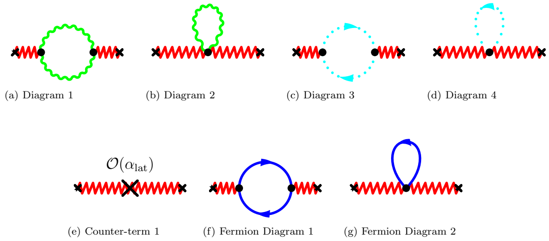
Figure 5.1: One loop Background field diagrams. Figure (e) is a one-loop counter-term from \mathcal{O}(\alpha_{\text{lat}}) corrections in the action (2.6).
