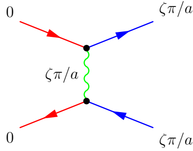
Figure 3.1: Generic tree-level taste-changing diagram for massless naïve quarks exchanging a hard gluon of momenta \zeta\pi/a .
