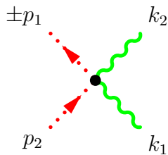
(g) Two-Gluon - Ghost Vertex. (A.53) on page 130.
