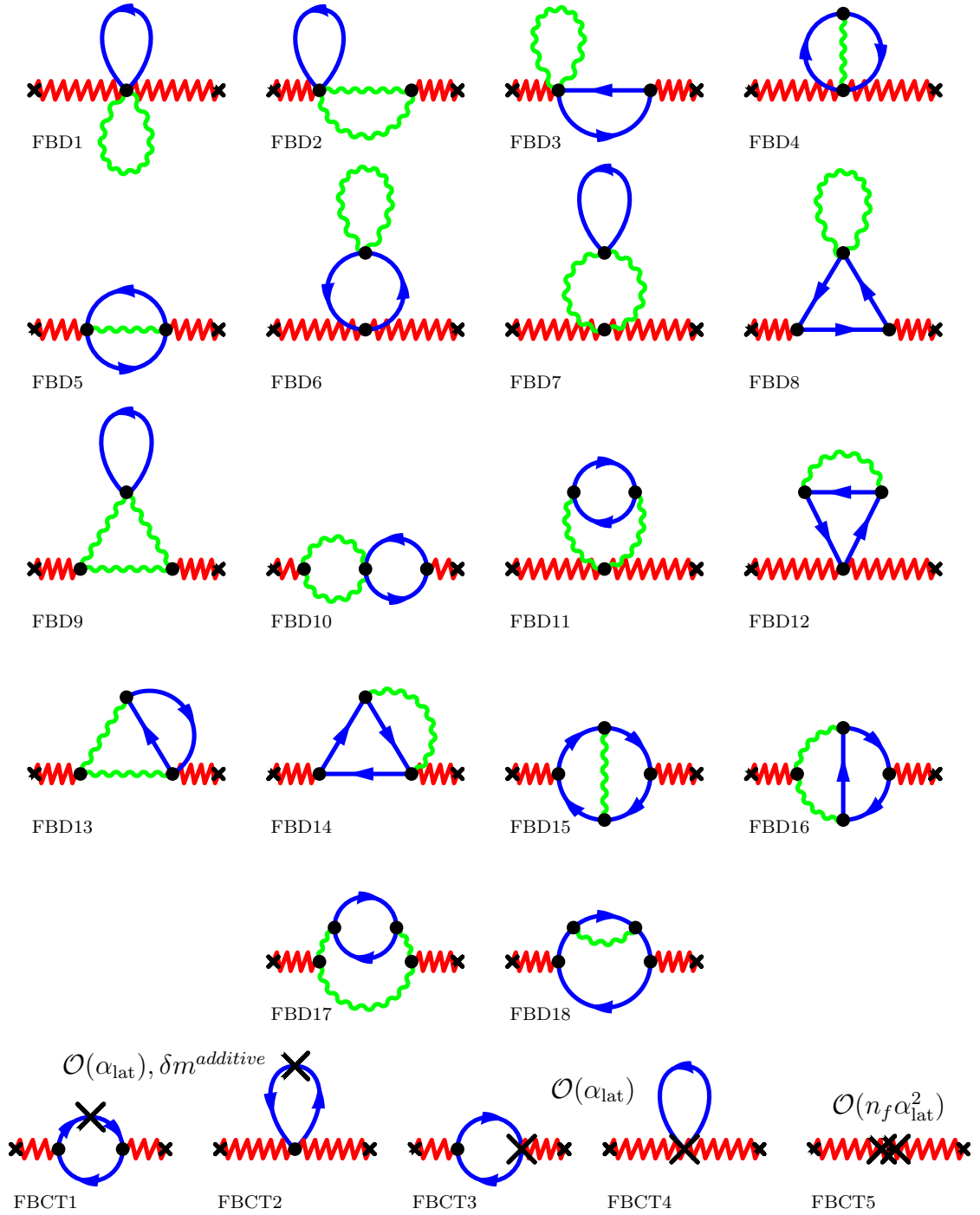
Figure 5.3: Two-loop F ermionic B ackground field D iagrams. The numbering scheme comes from [69]. After combining 7+11 and 9+17 everything is IR finite. 15-18 are the 4 continuum diagrams, and the last row are one- and two-loop lattice counter-term diagrams from (2.6).
