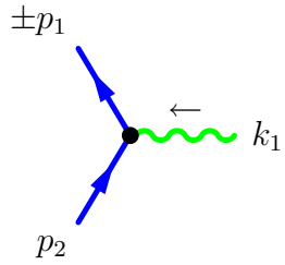
(b) One Gluon - Quark Vertex. (A.46) on page 128.
