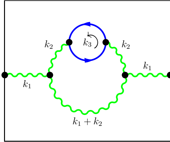
Figure 2.3: The Feynman diagram for the example being “automatically” generated. It can be tagged by (2.49), and has a final symmetry factor of -144/144=-1 just like the continuum.
