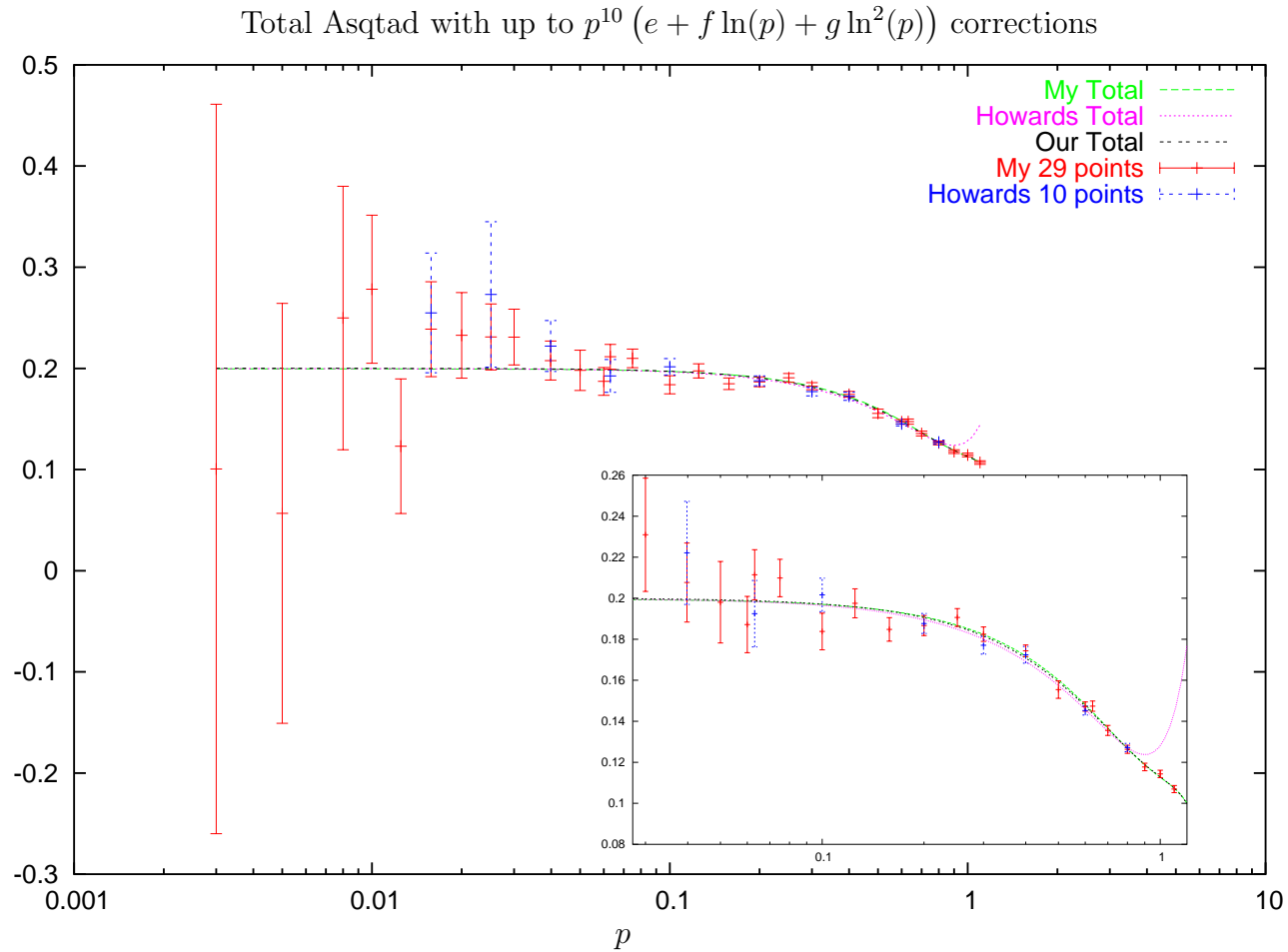
Figure 5.5: The final fit for the constant in \nu_{\text{lat}}^{(2)} = \sum_i c_{4,i} + \beta_1 \ln p , after the known logarithm, \beta_1 was subtracted out, shown over the complete range of external momenta calculated for the Asqtad action. Inset shows that data for p \sim 0.1 controls the quality of the final fit, and the agreement between the two independent evaluations.
