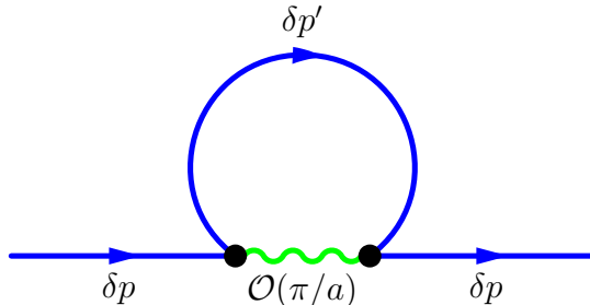
Figure 2.1: A quark tadpole that dominates quark diagrams for unimproved staggered quarks.
