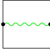
Figure 5.6: One-loop Feynman diagram for the expectation of a Wilson loop.
