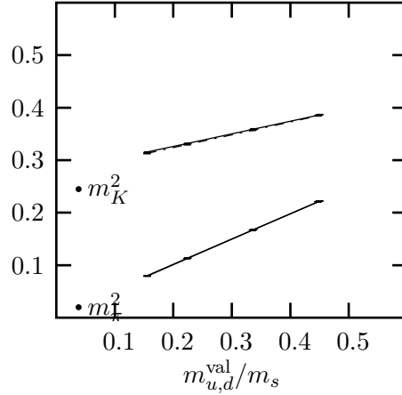
Figure 4.1: Chiral fits of m_\pi^2 and m_K^2 versus m_{u,d} (all in GeV) on the fine lattice before interpolation in m_s . The valence and sea quark s -quark masses are am_s = 0.031 (16% too high).
