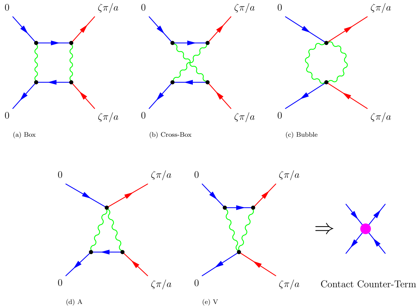
Figure 3.2: The five Feynman diagrams contributing to one-loop taste-changing for improved staggered quarks. Note that 15 other diagrams vanish due to the smearing in improved staggered.
