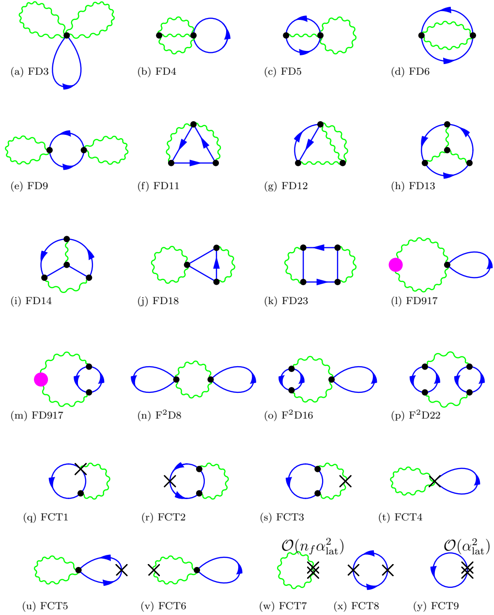
Figure 5.9: The three-loop fermionic Feynman diagrams for the expectation of a Wilson loop, evaluated from derivatives of vacuum bubbles using the susceptibility method (5.45). The diagram numbering is consistent with [69] except this D917=D7+D10+D15+D19+D25 and this D97=D17+D20+D21+D24+D26 . The notation F^2DX indicates that diagram X is proportional to n_f^2 rather than n_f , and CT indicates lattice counter-term. FCT8 and FCT9 are identically zero.
