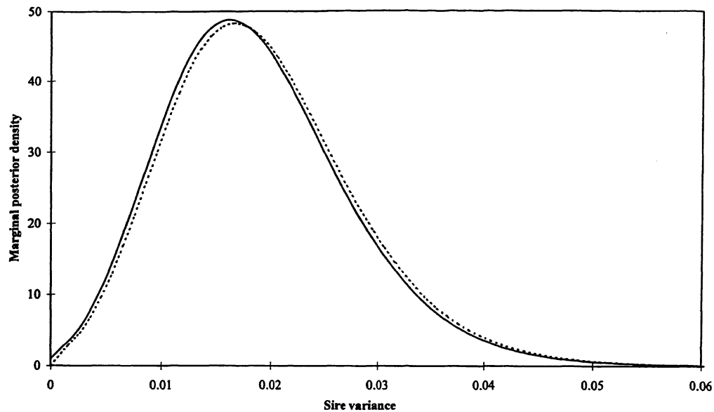
Fig 6. Marginal posterior density of the sire variance \sigma_s^2 obtained after Laplacian integration when a Weibull (—) or a Cox (- - - -) model is used; 5 000 records generated from a Weibull distribution; 100 sires with 50 daughters each; 100 'herd' effects; no censoring; \sigma_s^2 = 0.02 = \text{true value} .
