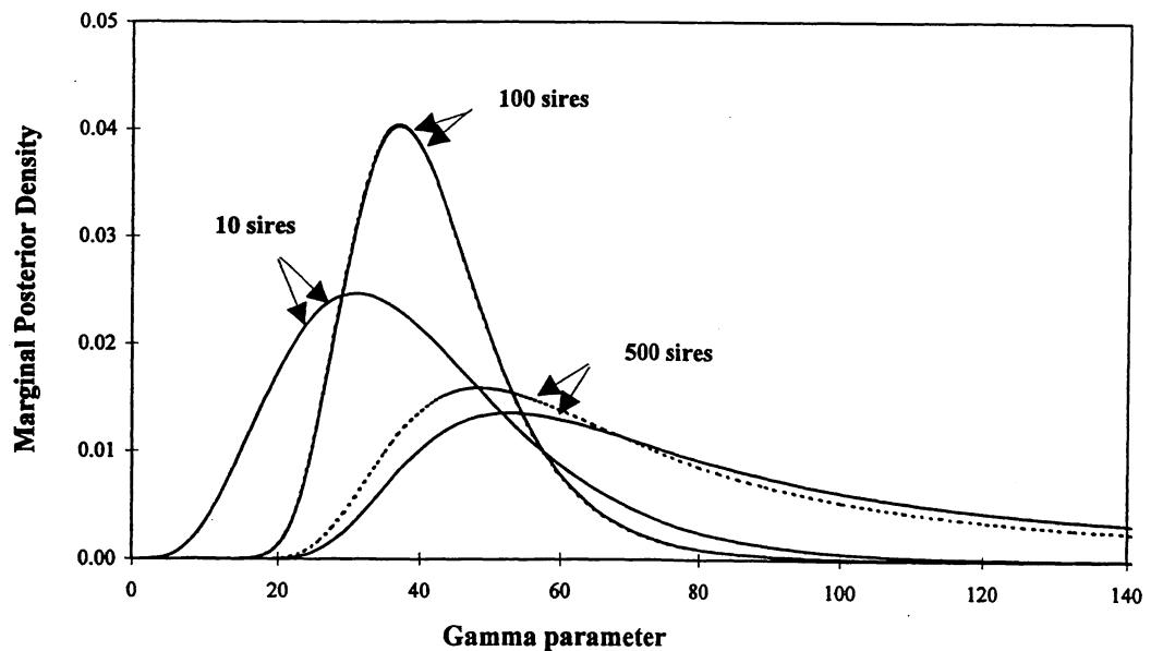
Fig 1. Marginal posterior density of the variance parameter \gamma obtained after Laplacian integration (---) or algebraic integration (—); 5 000 records; 10, 100 or 500 sires with 500, 50 or 10 daughters each. No censoring. \gamma = 50 = true value of the gamma parameter.
