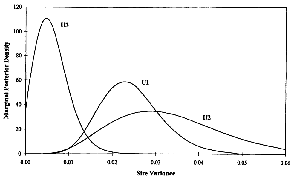
Fig 4. Marginal posterior density of the sire variance \sigma_s^2 obtained after Laplacian integration in three unbalanced cases; 5 000 records. Case U1: 500 herds with five animals; five herds with 500 animals. Case U2: 500 sires with five daughters each; five sires with 500 daughters each. Case U3: the daughters of the best sires are located in the best herds. No censoring; \sigma_s^2 = 0.02 = \text{true value} .
