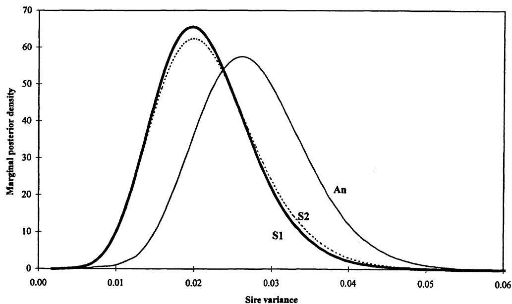
Fig 5. Marginal posterior density of the sire variance \sigma_s^2 obtained after Laplacian integration under two sire models (without a relationship matrix (S1) or with the true relationship matrix between sires (S2)) and under an animal model (An); 5 000 records; no censoring; \sigma_s^2 = 0.02 = \text{true value} .
